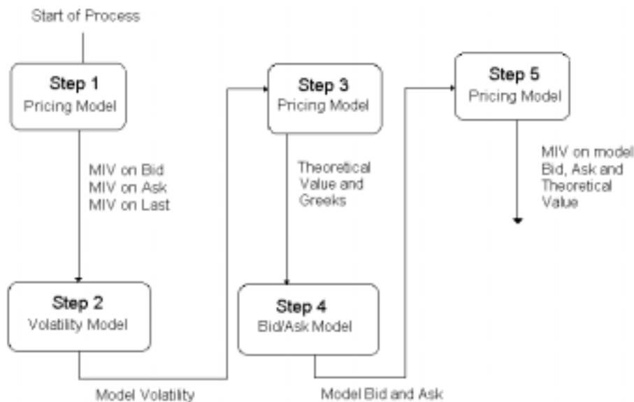
Figure 5-10. OptionStation Five-Step Pricing Model Engine
