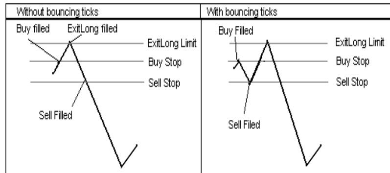
Figure 3-12. Bouncing tick example
