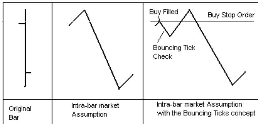
Figure 3-11. Bouncing tick
