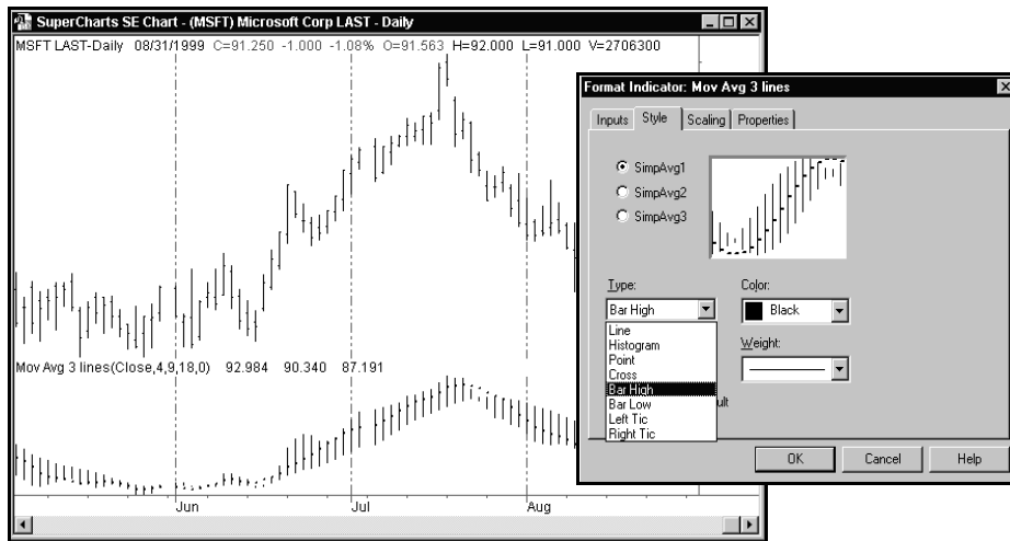
Figure 5-5. Indicator formatted to display as a bar chart
